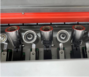
Chrome Steel straight and bevel pressure rollers
