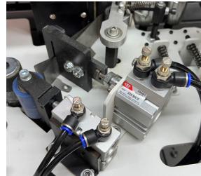
Pneumatic Tape guillotine
