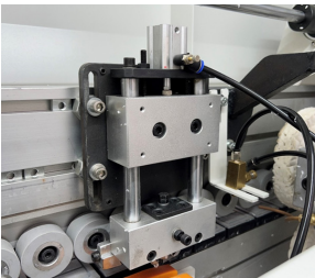
Top and bottom Flat Glue Scrapers
